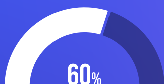
Change Coverage
